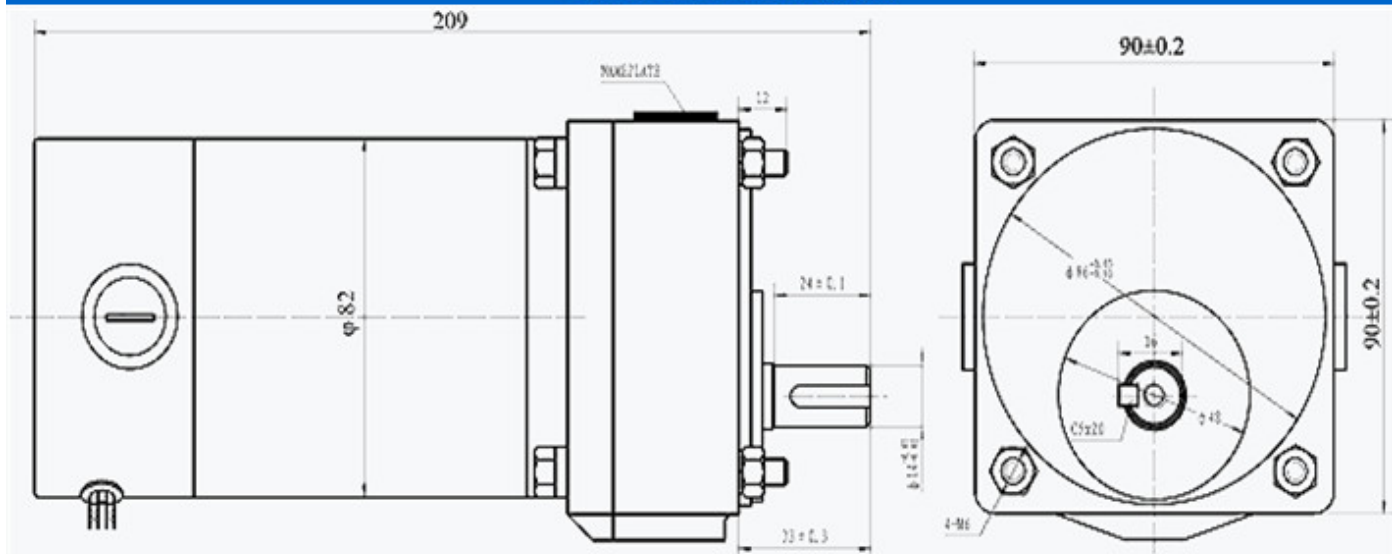
Outline Drawing/外形圖
